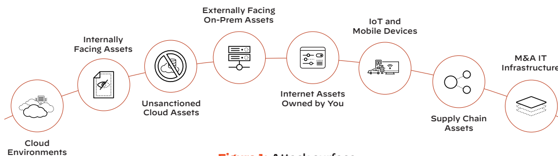
Figure 1: Attack surface
