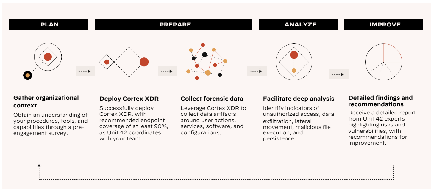
Figure 1: Methodology
